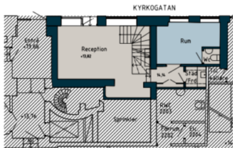
PLAN 2, GATUPLAN
